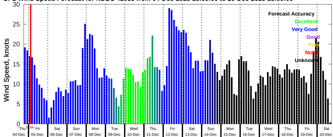
GFS Wind Speed Forecast for NDBC 42035 from 04-Dec-2025 18:00:00 to 20-Dec-2025 18:00:00
