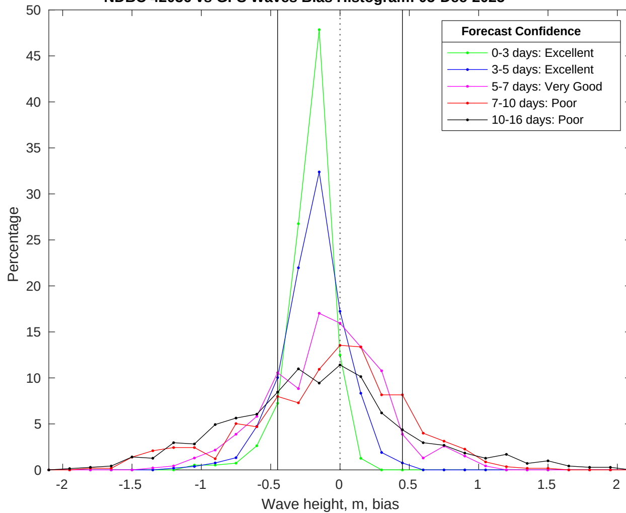
NDBC 42036 vs GFS Waves Bias Histogram: 05-Dec-2025
