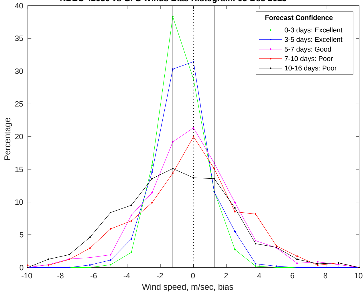
NDBC 42036 vs GFS Winds Bias Histogram: 05-Dec-2025
