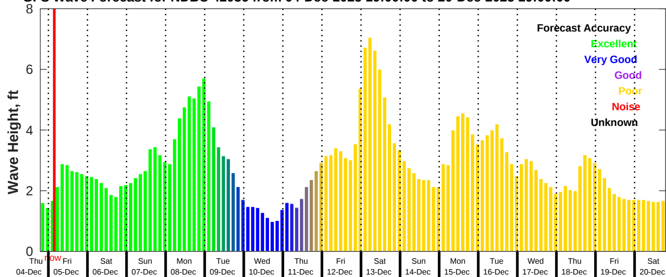
GFS Wave Forecast for NDBC 42036 from 04-Dec-2025 19:00:00 to 20-Dec-2025 19:00:00
