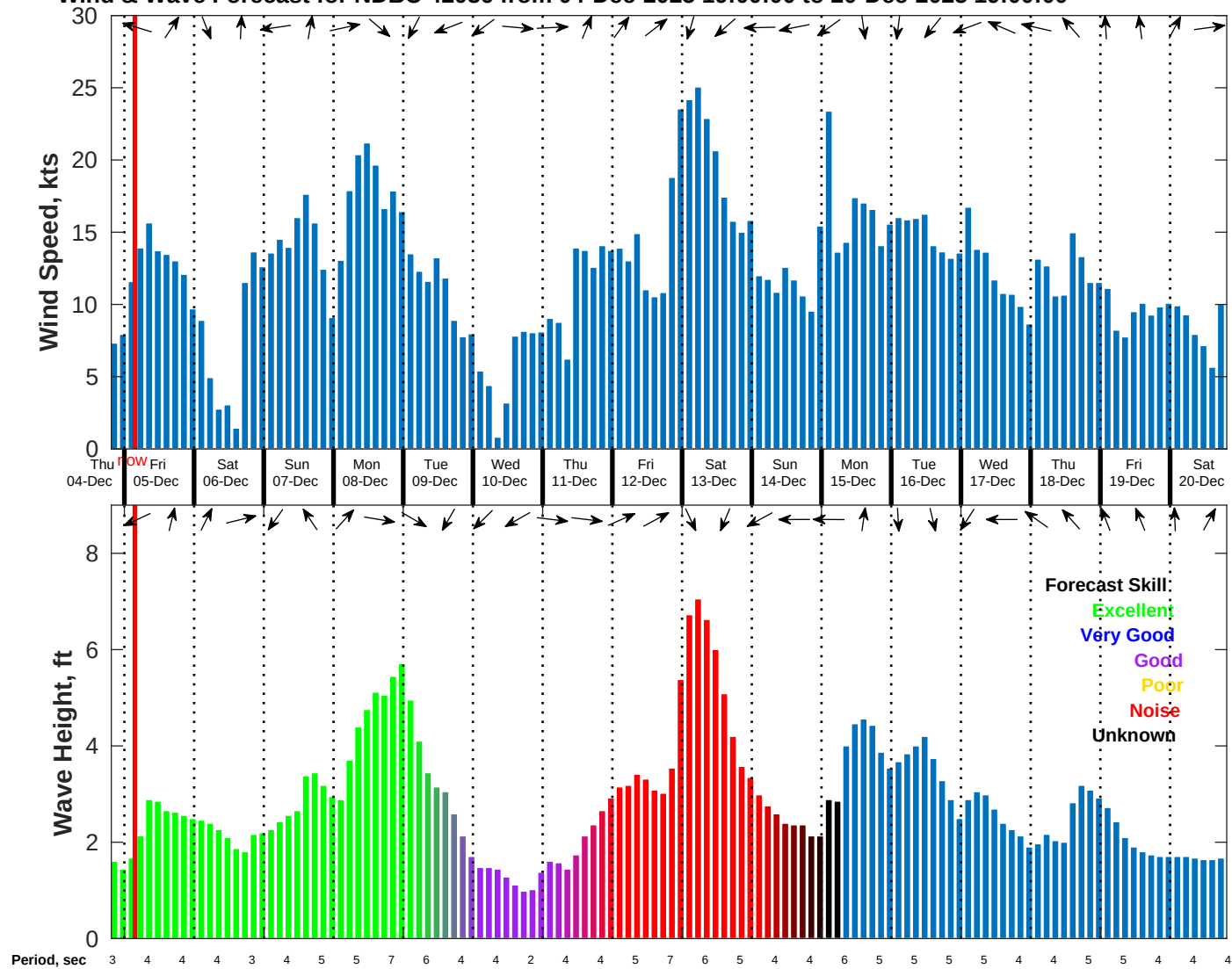
Wind & Wave Forecast for NDBC 42036 from 04-Dec-2025 19:00:00 to 20-Dec-2025 19:00:00
