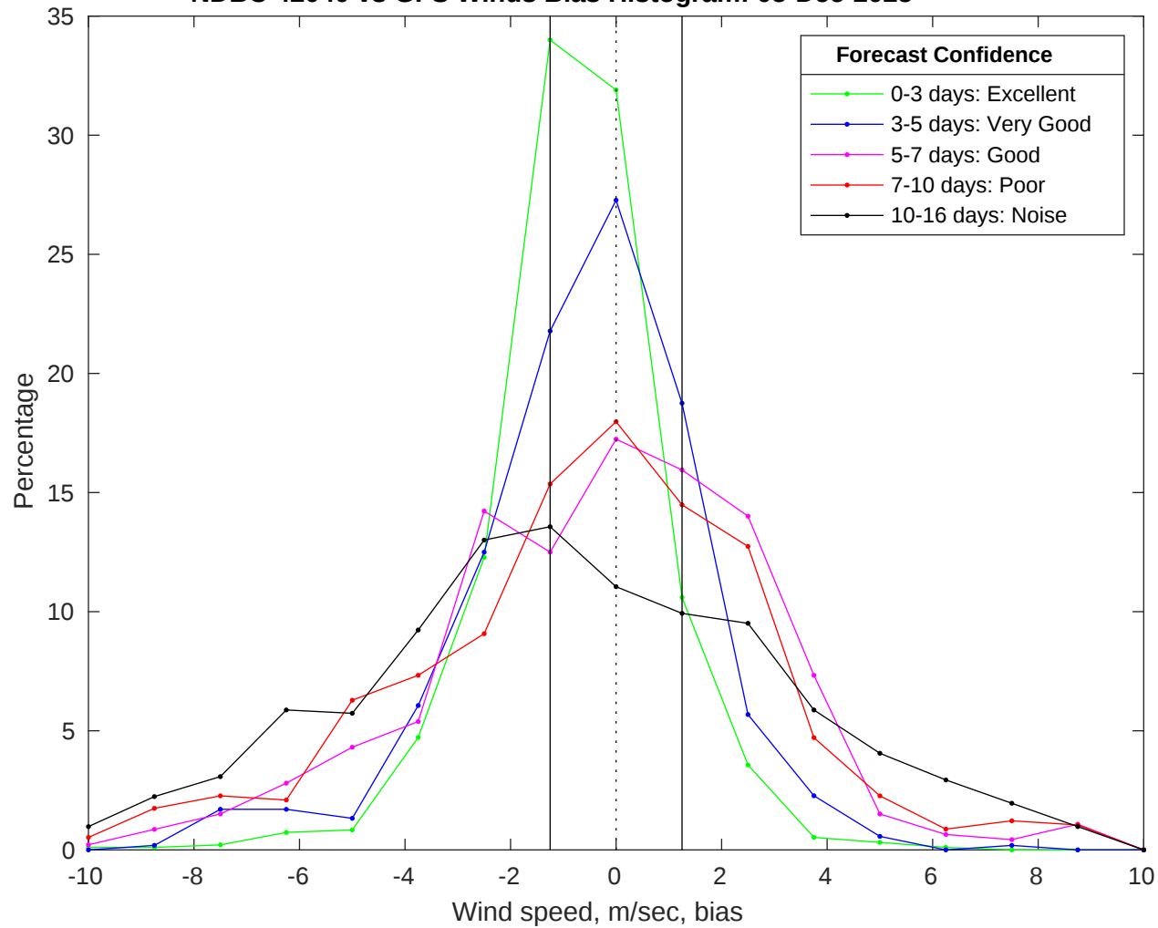
NDBC 42040 vs GFS Winds Bias Histogram: 05-Dec-2025
