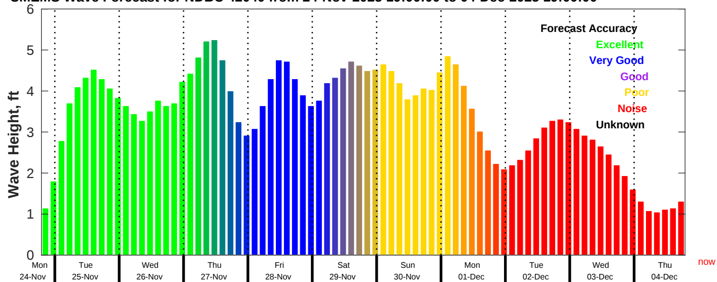
CMEMS Wave Forecast for NDBC 42040 from 24-Nov-2025 19:00:00 to 04-Dec-2025 19:00:00
