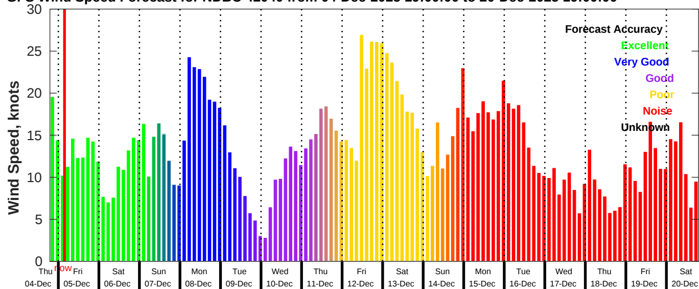
GFS Wind Speed Forecast for NDBC 42040 from 04-Dec-2025 19:00:00 to 20-Dec-2025 19:00:00
