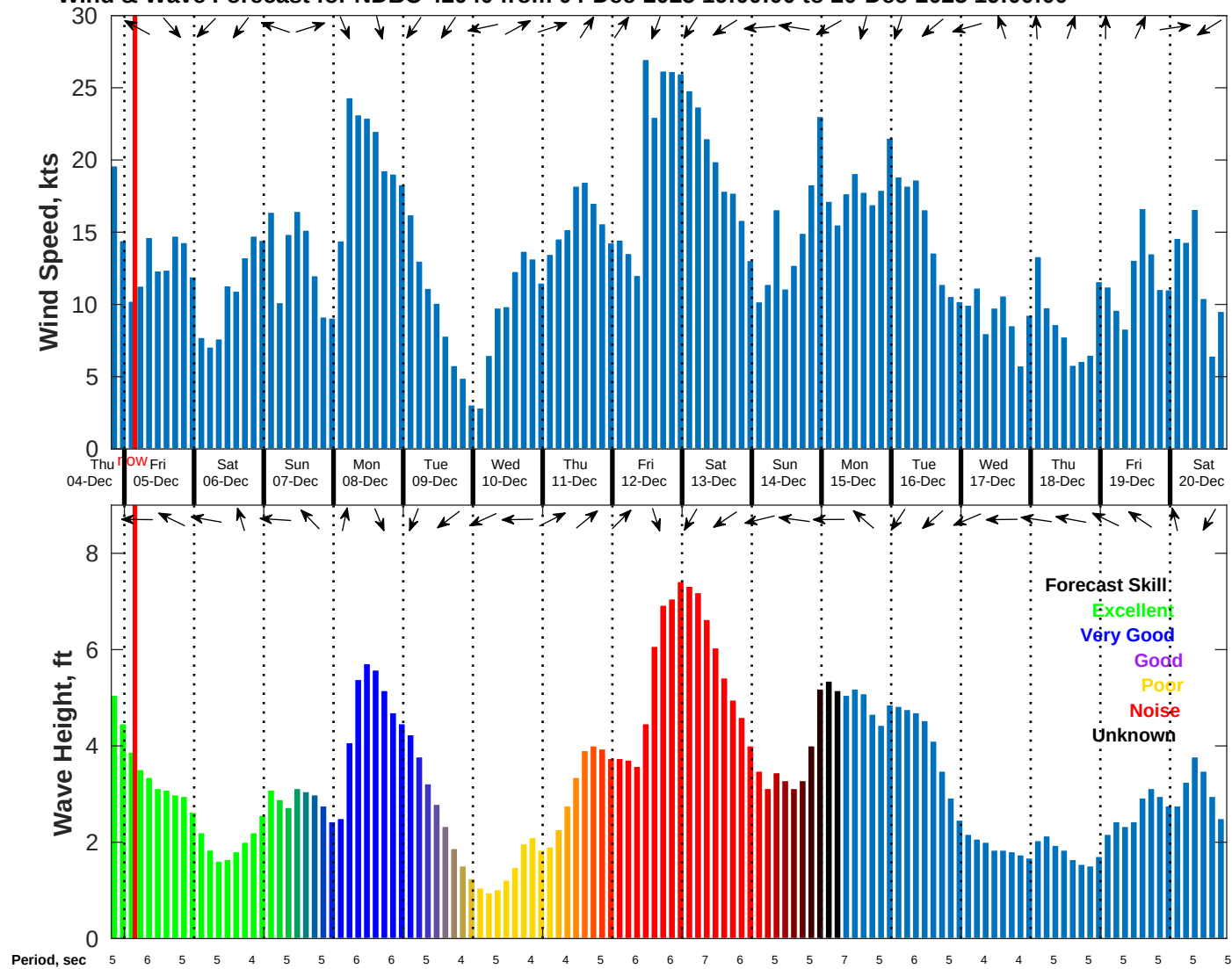
Wind & Wave Forecast for NDBC 42040 from 04-Dec-2025 19:00:00 to 20-Dec-2025 19:00:00
