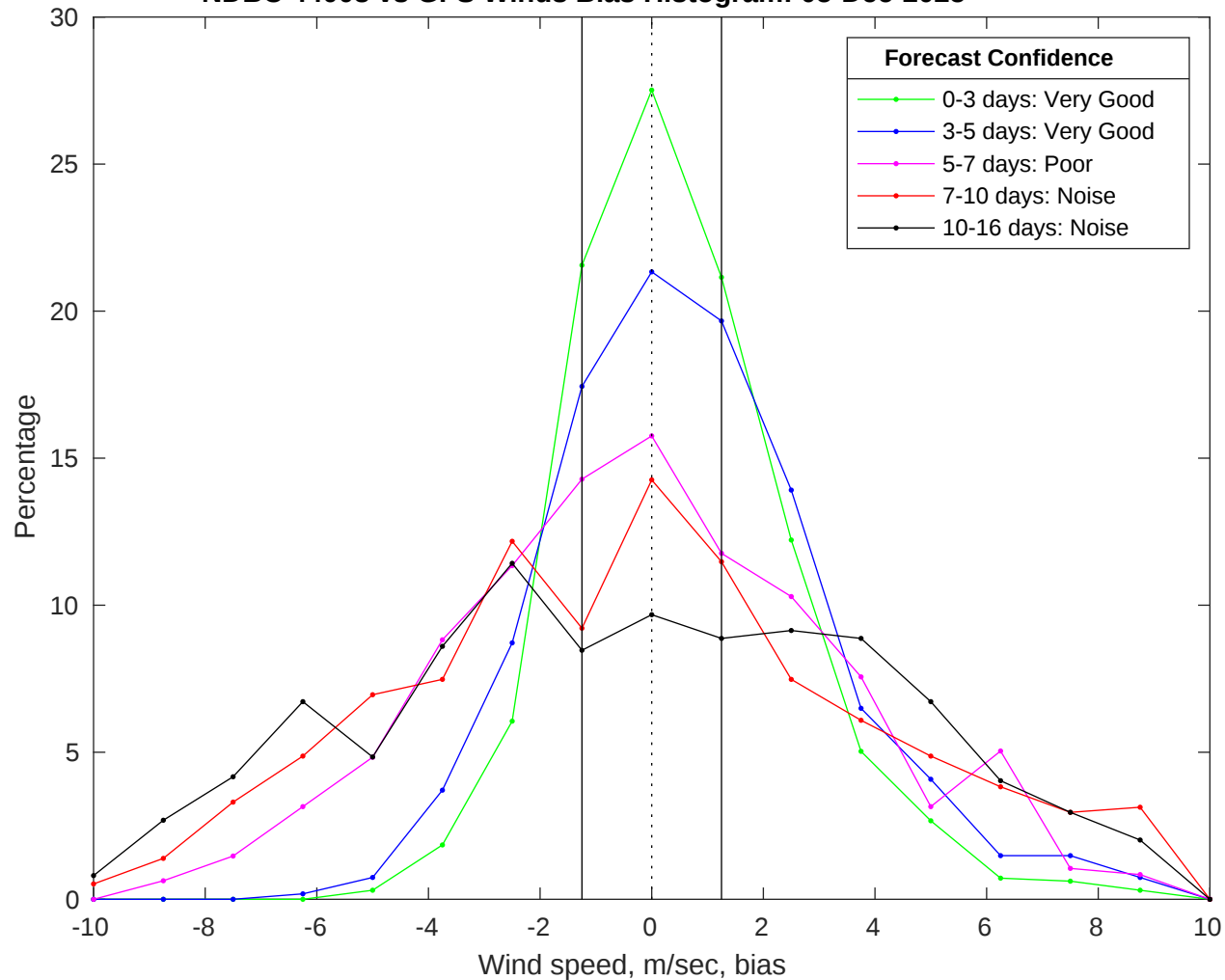
NDBC 44008 vs GFS Winds Bias Histogram: 05-Dec-2025
