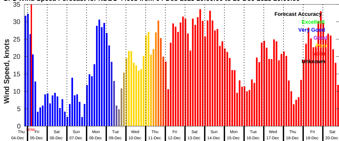
GFS Wind Speed Forecast for NDBC 44008 from 04-Dec-2025 20:00:00 to 20-Dec-2025 20:00:00
