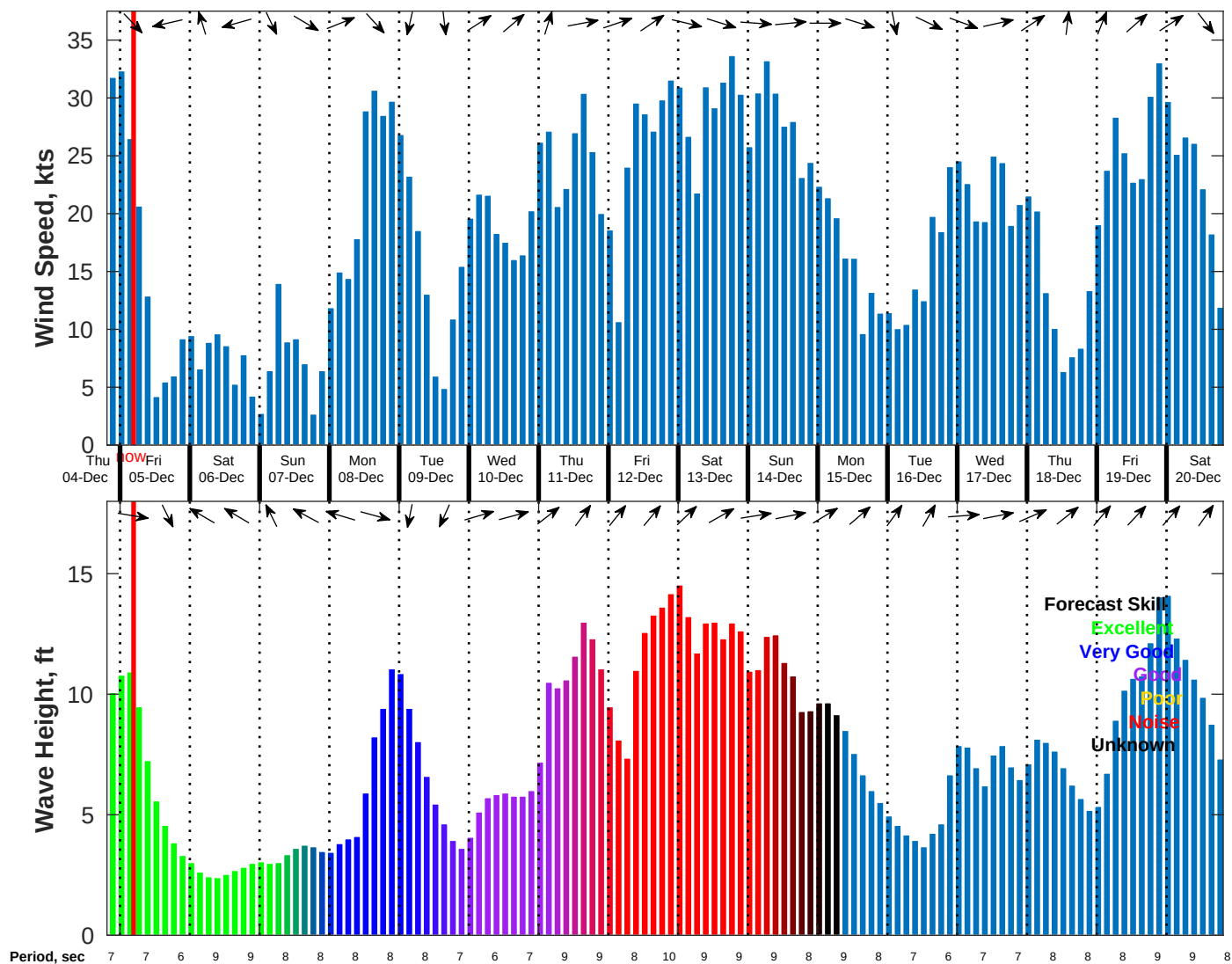
Wind & Wave Forecast for NDBC 44008 from 04-Dec-2025 20:00:00 to 20-Dec-2025 20:00:00
