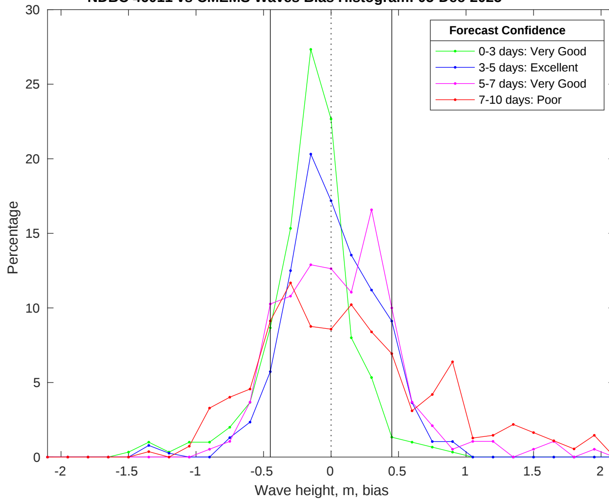
NDBC 46011 vs CMEMS Waves Bias Histogram: 05-Dec-2025
