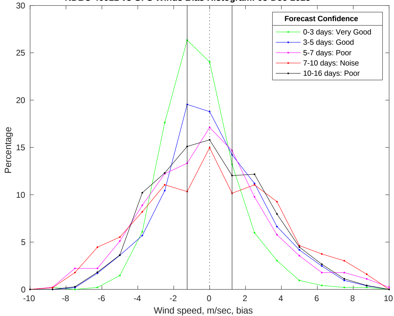
NDBC 46011 vs GFS Winds Bias Histogram: 05-Dec-2025
