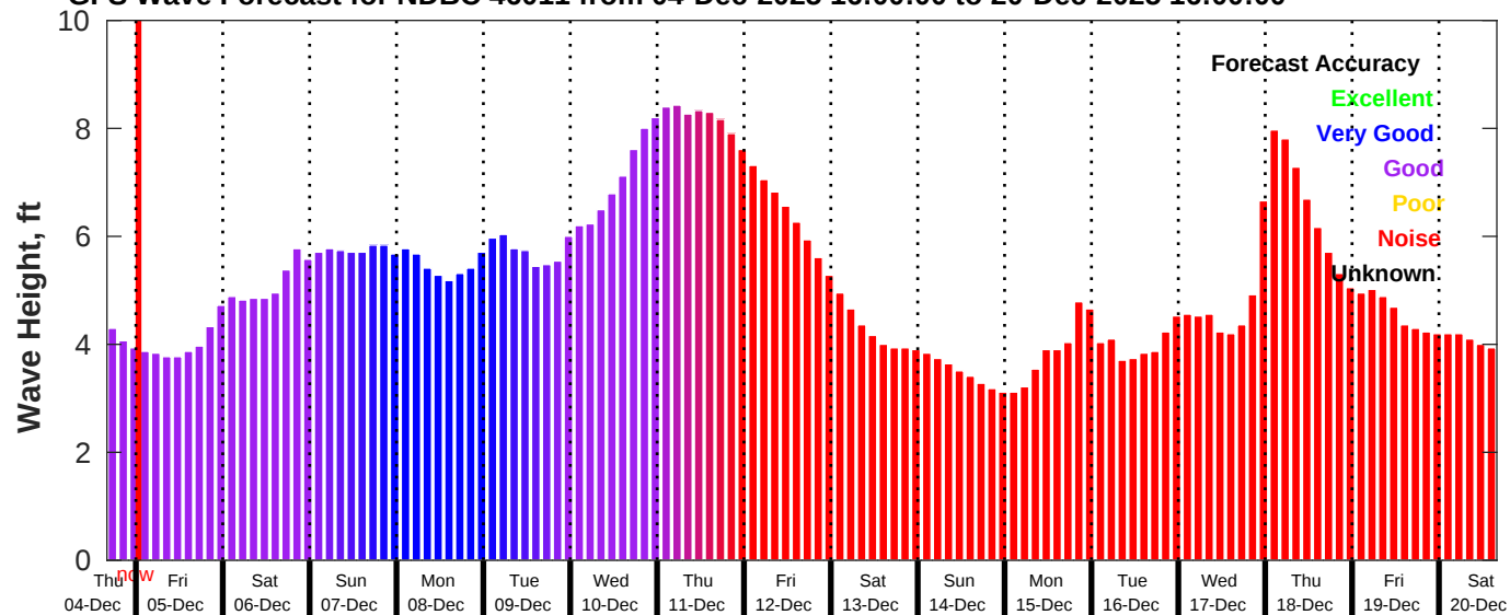
GFS Wave Forecast for NDBC 46011 from 04-Dec-2025 16:00:00 to 20-Dec-2025 16:00:00
