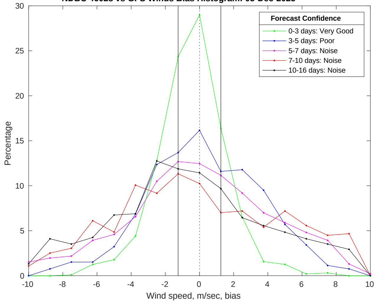
NDBC 46028 vs GFS Winds Bias Histogram: 05-Dec-2025
