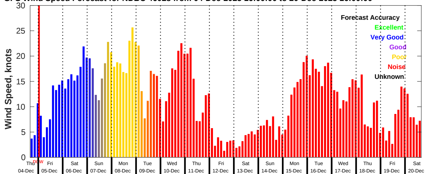
GFS Wind Speed Forecast for NDBC 46028 from 04-Dec-2025 16:00:00 to 20-Dec-2025 16:00:00
