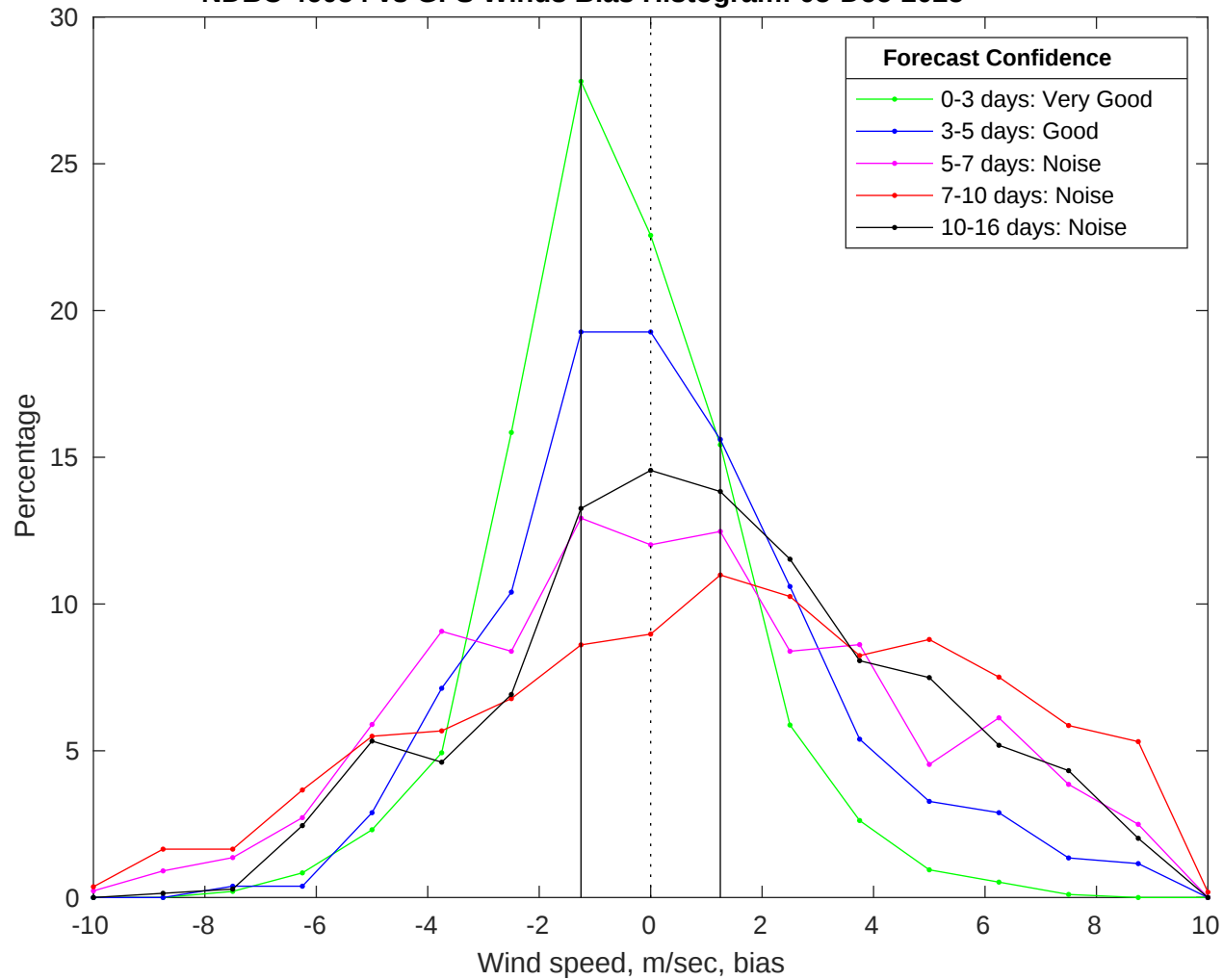
NDBC 46054 vs GFS Winds Bias Histogram: 05-Dec-2025
