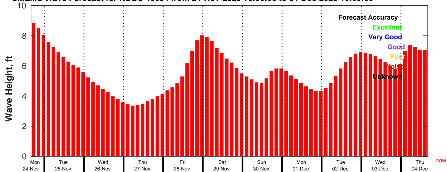
CMEMS Wave Forecast for NDBC 46054 from 24-Nov-2025 16:00:00 to 04-Dec-2025 16:00:00
