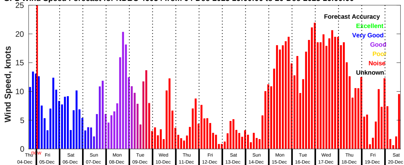
GFS Wind Speed Forecast for NDBC 46054 from 04-Dec-2025 16:00:00 to 20-Dec-2025 16:00:00
