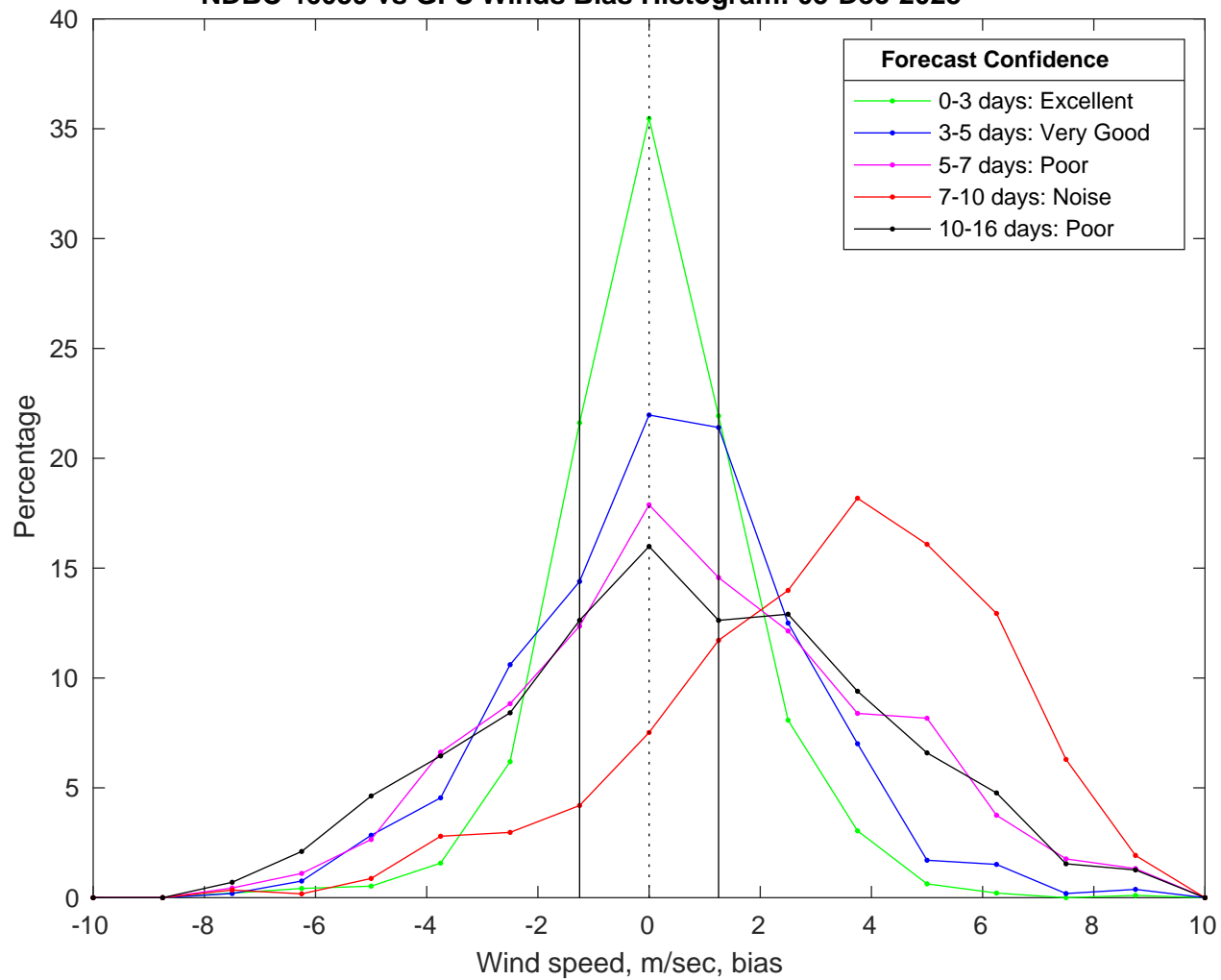
NDBC 46059 vs GFS Winds Bias Histogram: 05-Dec-2025
