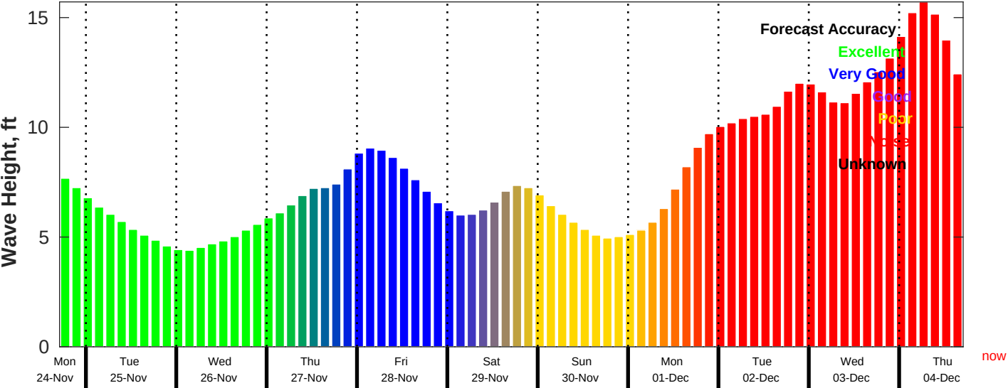
CMEMS Wave Forecast for NDBC 46059 from 24-Nov-2025 17:00:00 to 04-Dec-2025 17:00:00
