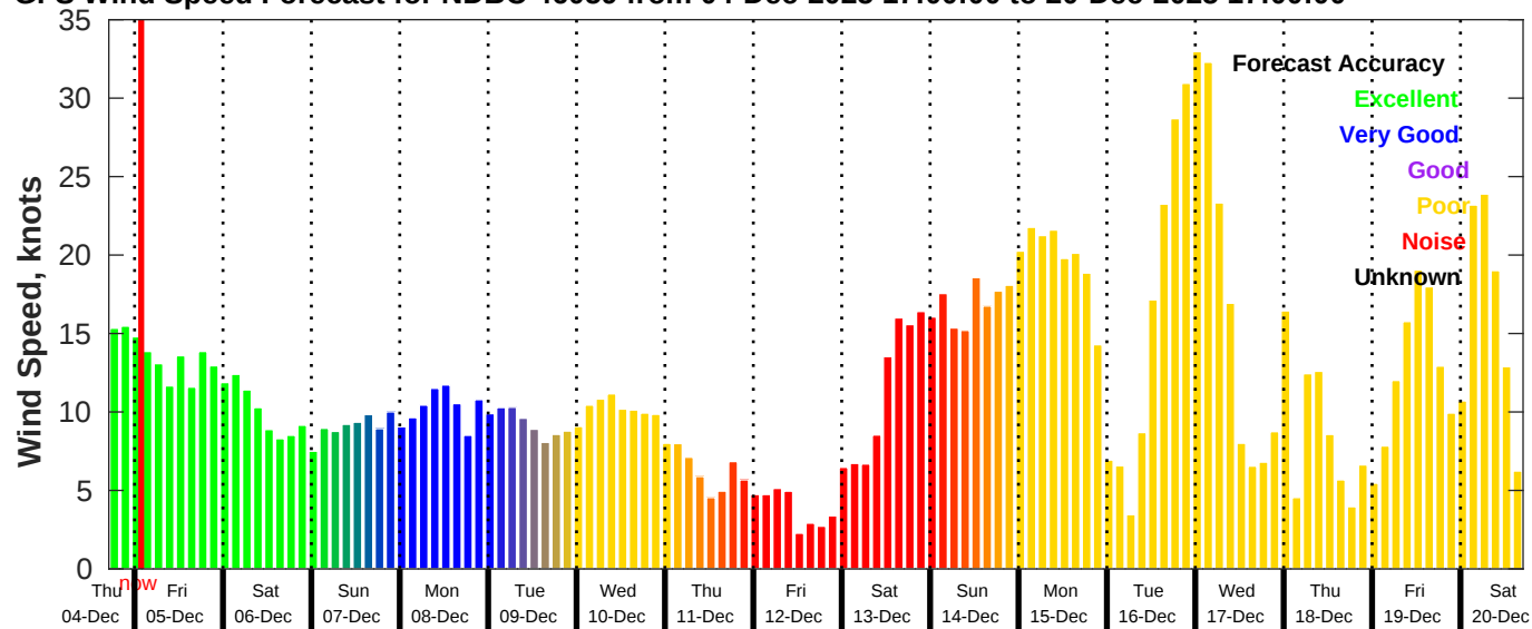
GFS Wind Speed Forecast for NDBC 46059 from 04-Dec-2025 17:00:00 to 20-Dec-2025 17:00:00
