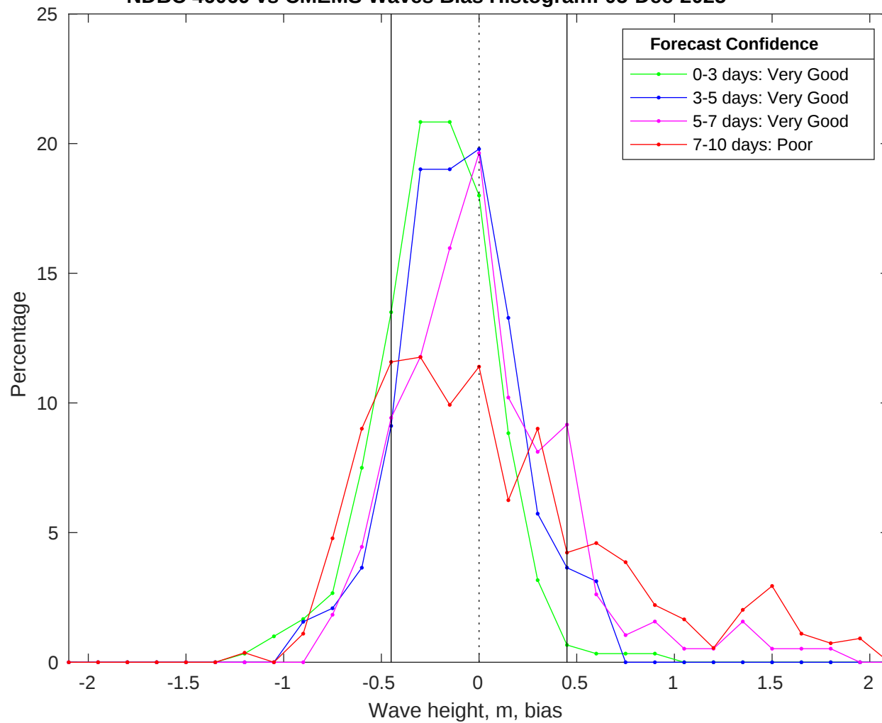
NDBC 46069 vs CMEMS Waves Bias Histogram: 05-Dec-2025
