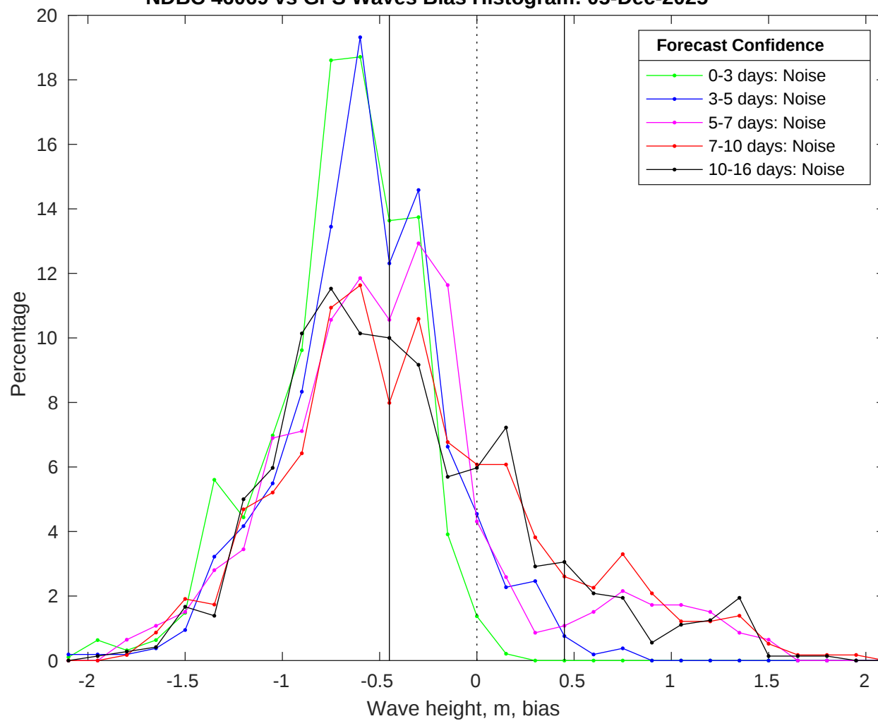
NDBC 46069 vs GFS Waves Bias Histogram: 05-Dec-2025
