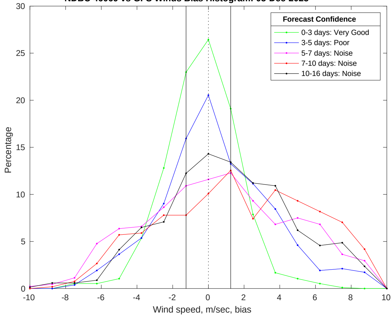
NDBC 46069 vs GFS Winds Bias Histogram: 05-Dec-2025
