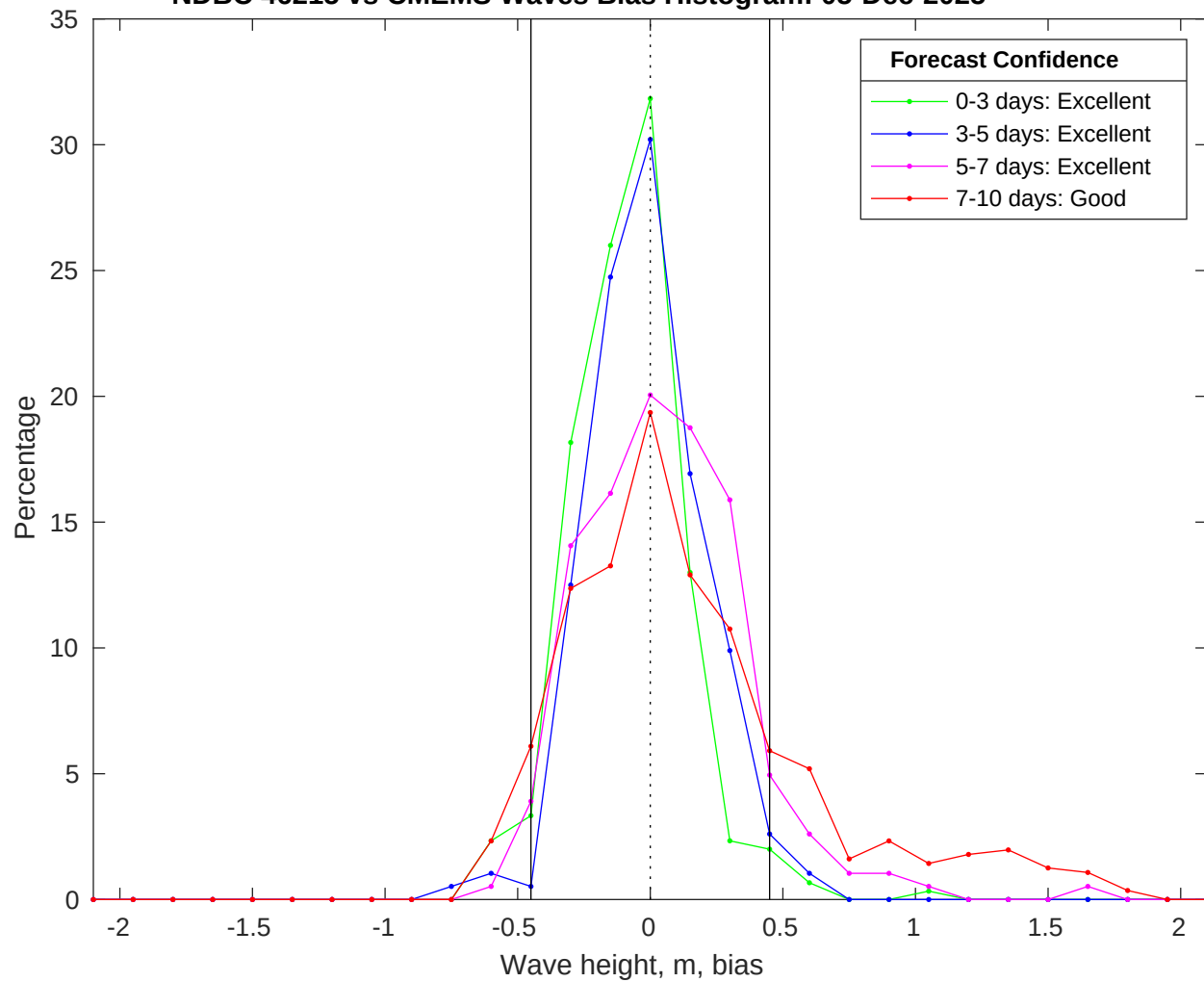
NDBC 46215 vs CMEMS Waves Bias Histogram: 05-Dec-2025
