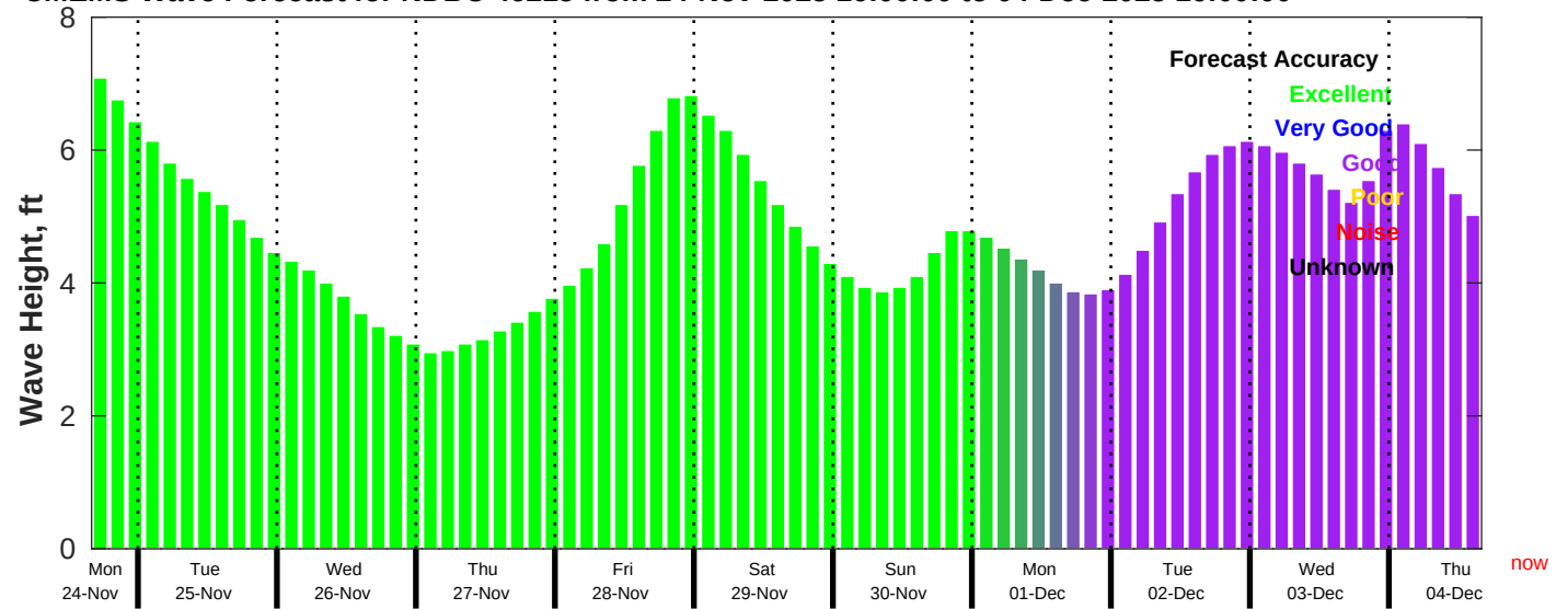
CMEMS Wave Forecast for NDBC 46215 from 24-Nov-2025 16:00:00 to 04-Dec-2025 16:00:00
