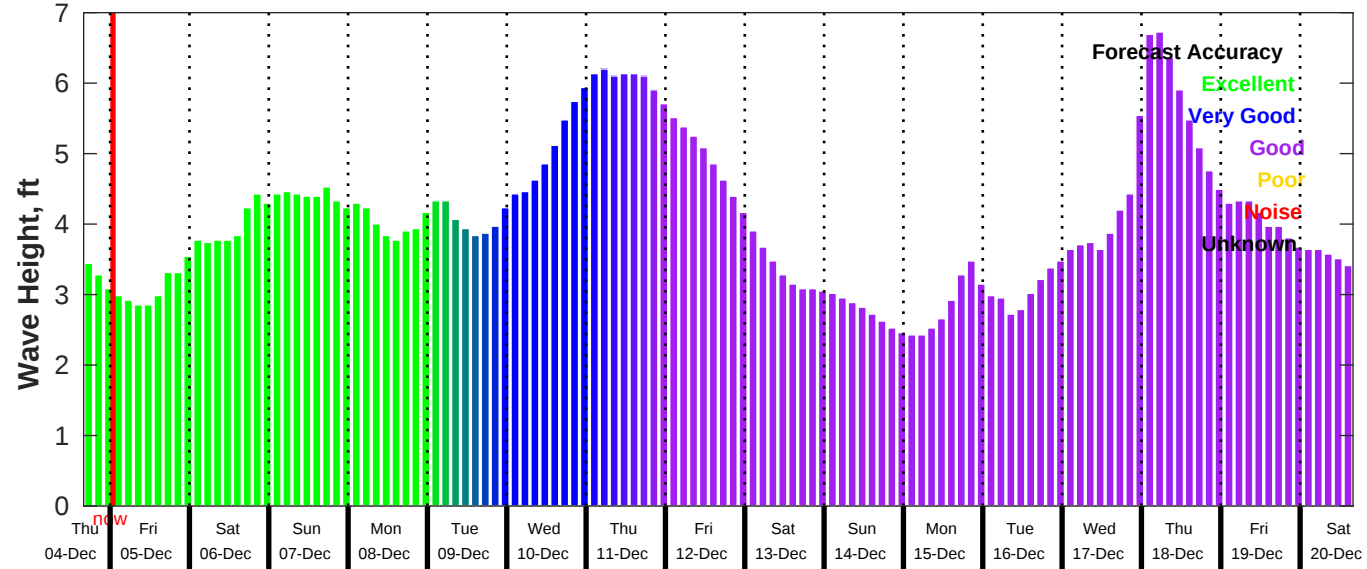
GFS Wave Forecast for NDBC 46215 from 04-Dec-2025 16:00:00 to 20-Dec-2025 16:00:00
