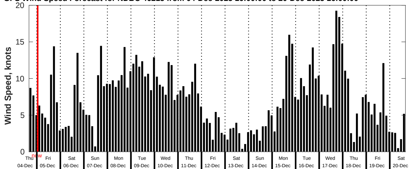
GFS Wind Speed Forecast for NDBC 46215 from 04-Dec-2025 16:00:00 to 20-Dec-2025 16:00:00
