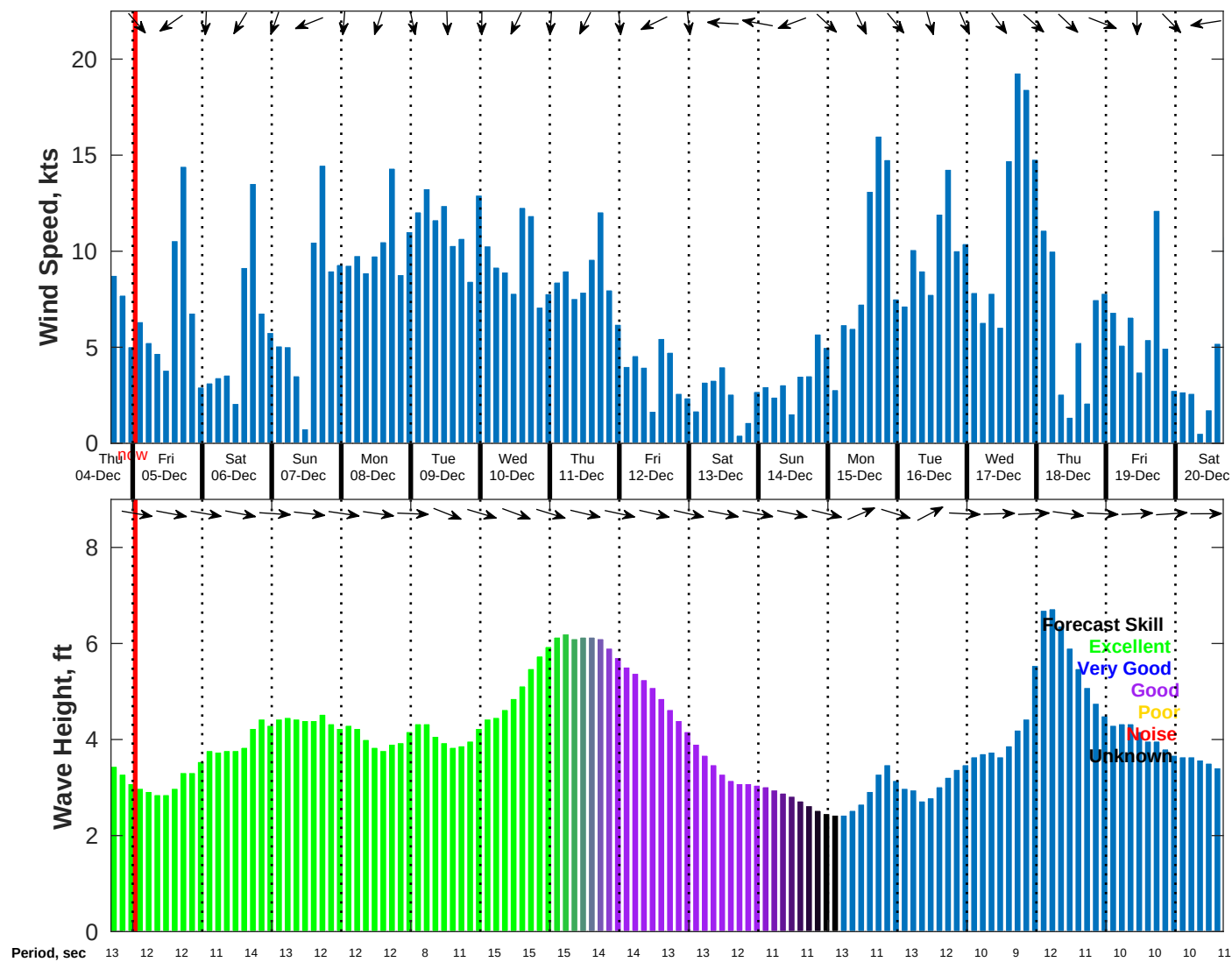
Wind & Wave Forecast for NDBC 46215 from 04-Dec-2025 16:00:00 to 20-Dec-2025 16:00:00
