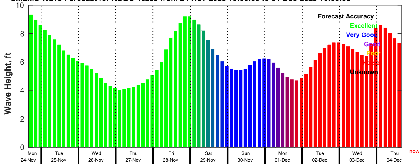
CMEMS Wave Forecast for NDBC 46259 from 24-Nov-2025 16:00:00 to 04-Dec-2025 16:00:00
