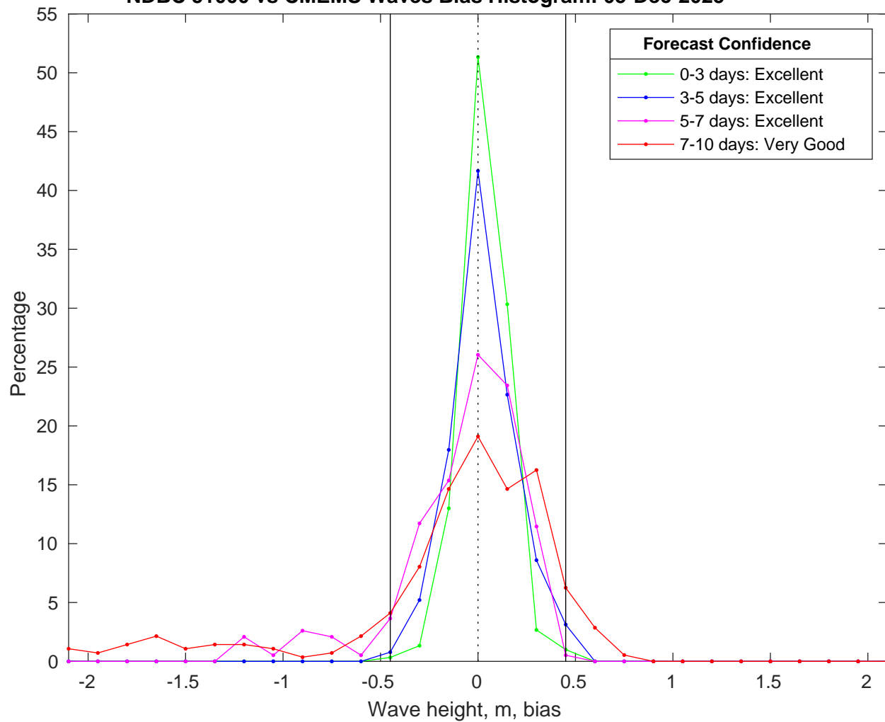
NDBC 51000 vs CMEMS Waves Bias Histogram: 05-Dec-2025
