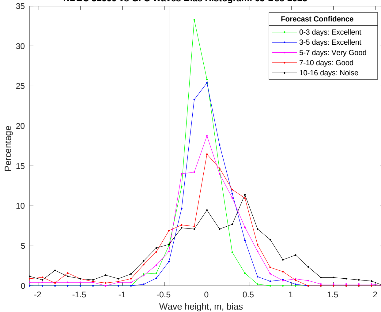
NDBC 51000 vs GFS Waves Bias Histogram: 05-Dec-2025
