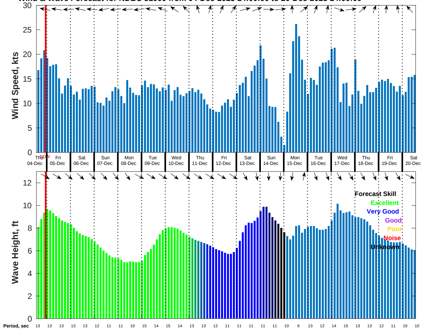
Wind & Wave Forecast for NDBC 51000 from 04-Dec-2025 14:00:00 to 20-Dec-2025 14:00:00
