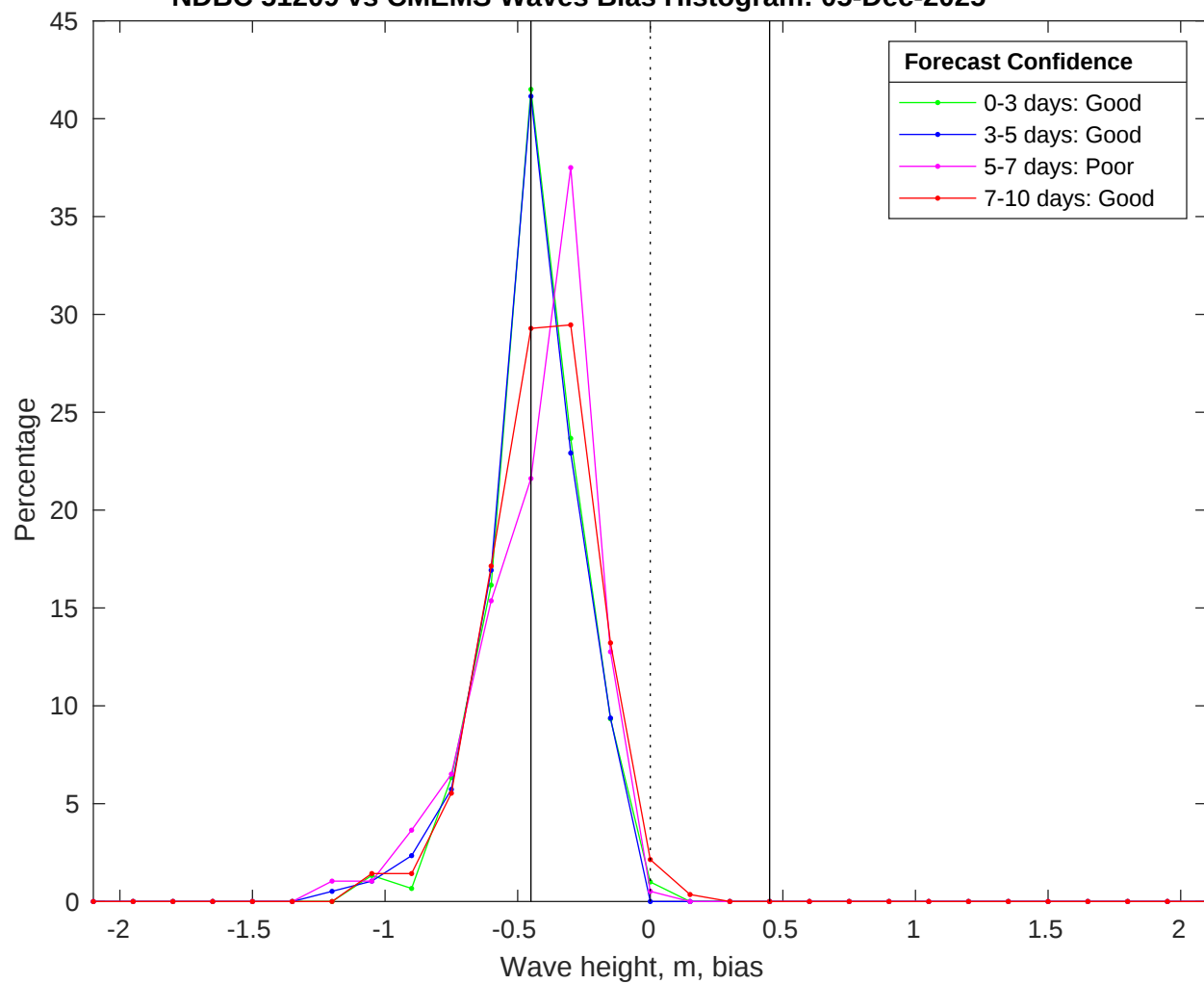
NDBC 51209 vs CMEMS Waves Bias Histogram: 05-Dec-2025
