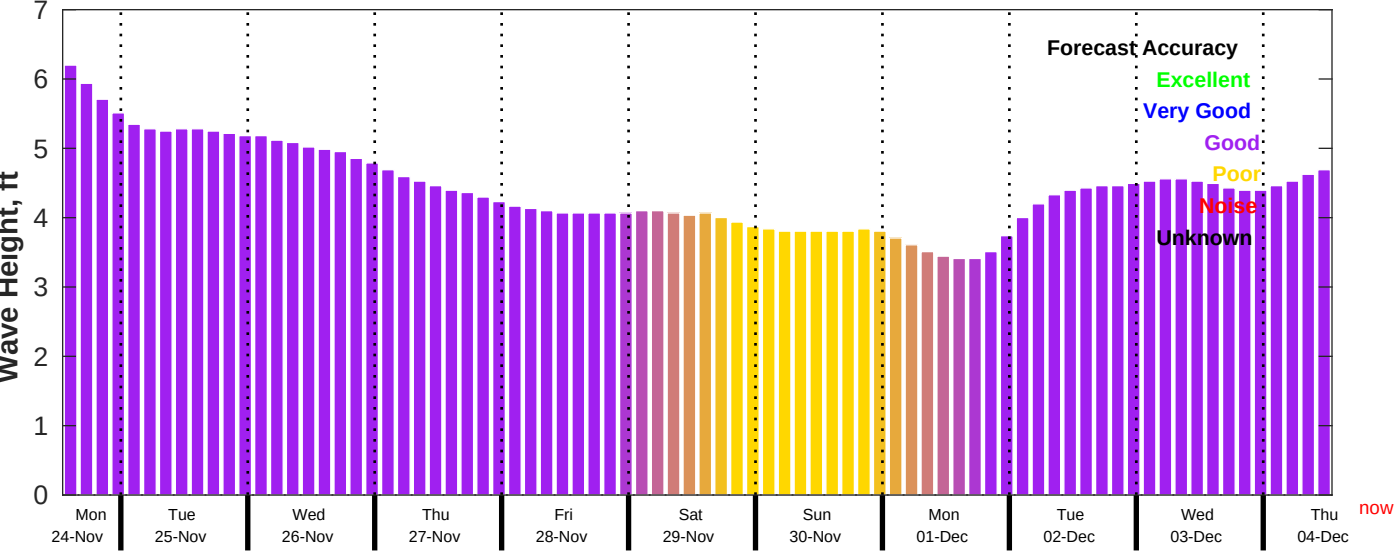
CMEMS Wave Forecast for NDBC 51209 from 24-Nov-2025 13:00:00 to 04-Dec-2025 13:00:00
