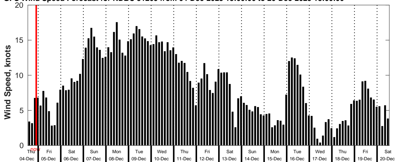
GFS Wind Speed Forecast for NDBC 51209 from 04-Dec-2025 13:00:00 to 20-Dec-2025 13:00:00
