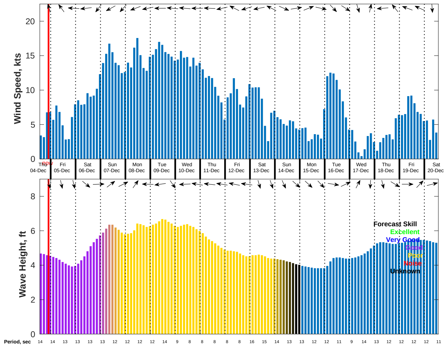
Wind & Wave Forecast for NDBC 51209 from 04-Dec-2025 13:00:00 to 20-Dec-2025 13:00:00
