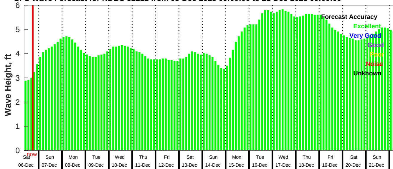
GFS Wave Forecast for NDBC 52212 from 05-Dec-2025 09:00:00 to 21-Dec-2025 09:00:00
