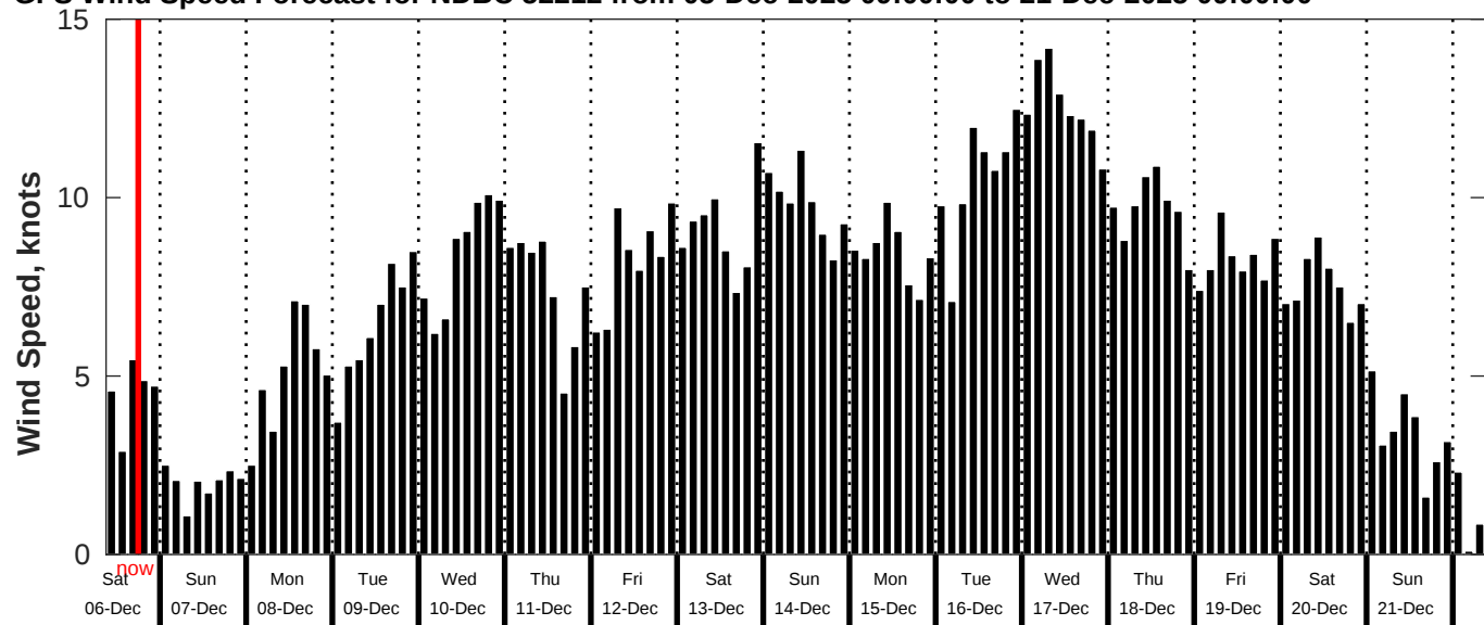
GFS Wind Speed Forecast for NDBC 52212 from 05-Dec-2025 09:00:00 to 21-Dec-2025 09:00:00
