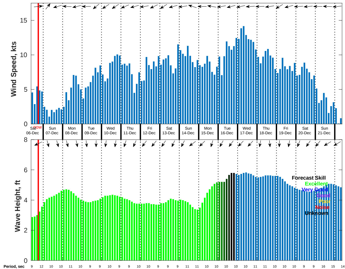
Wind & Wave Forecast for NDBC 52212 from 05-Dec-2025 09:00:00 to 21-Dec-2025 09:00:00
