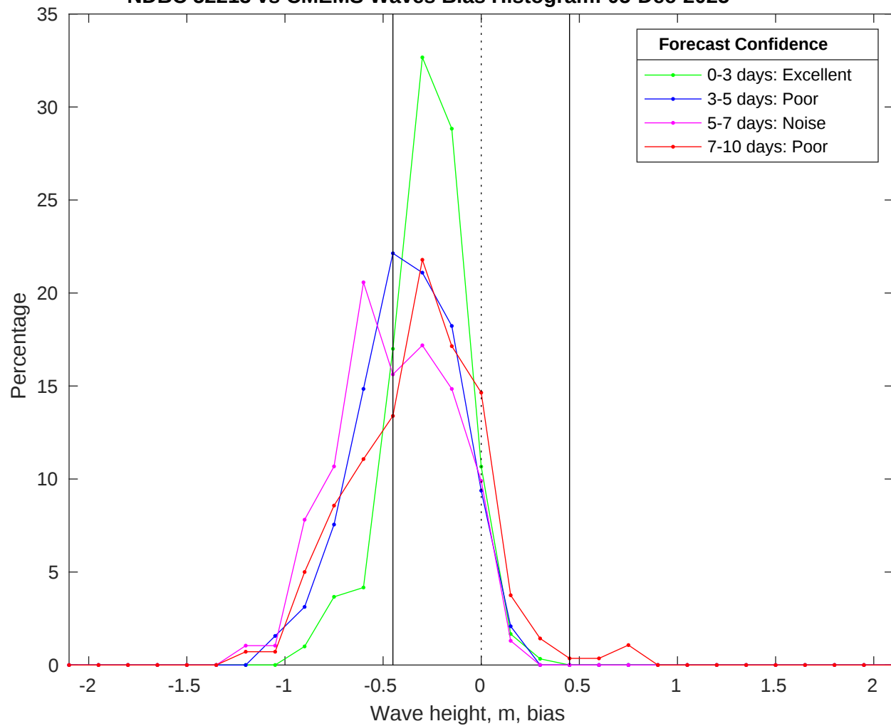
NDBC 52213 vs CMEMS Waves Bias Histogram: 05-Dec-2025
