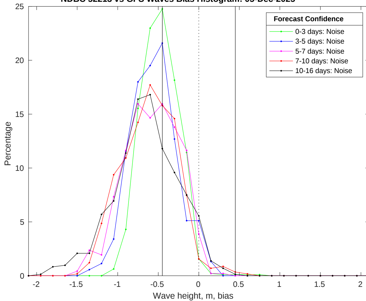
NDBC 52213 vs GFS Waves Bias Histogram: 05-Dec-2025
