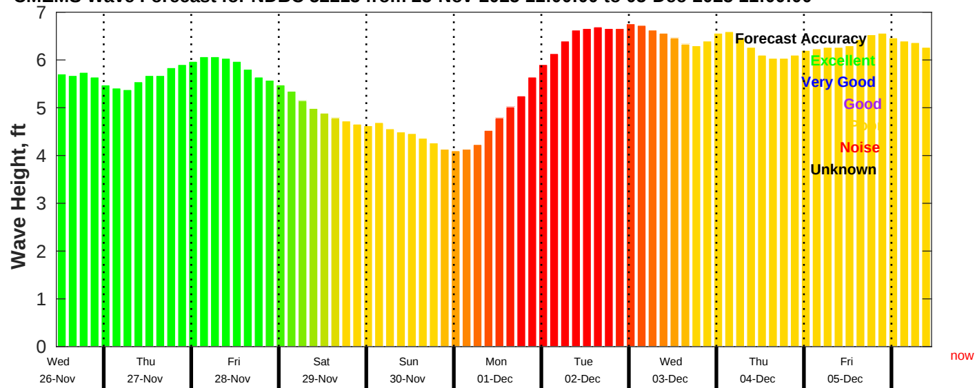
CMEMS Wave Forecast for NDBC 52213 from 25-Nov-2025 11:00:00 to 05-Dec-2025 11:00:00
