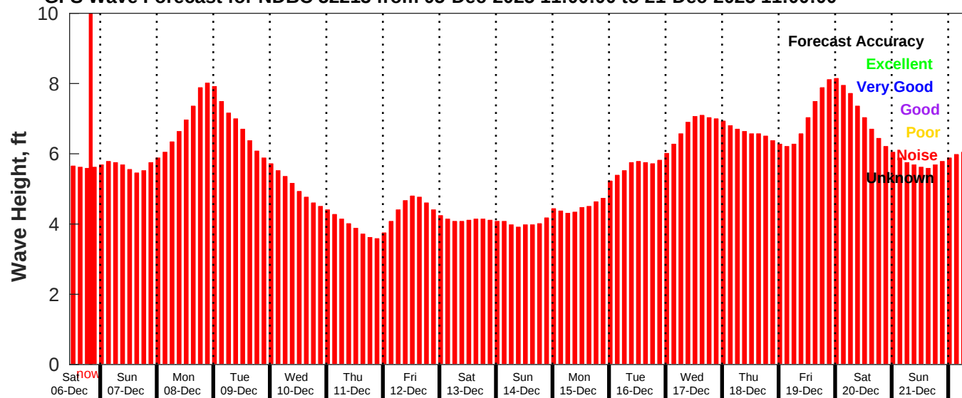
GFS Wave Forecast for NDBC 52213 from 05-Dec-2025 11:00:00 to 21-Dec-2025 11:00:00
