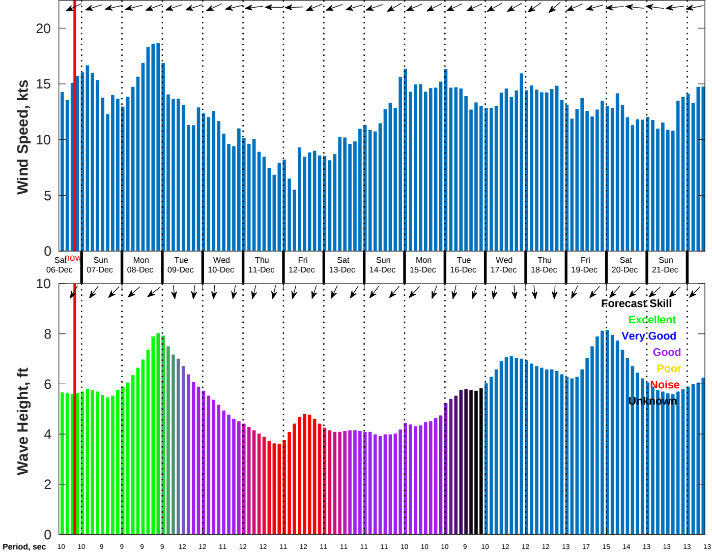
Wind & Wave Forecast for NDBC 52213 from 05-Dec-2025 11:00:00 to 21-Dec-2025 11:00:00
