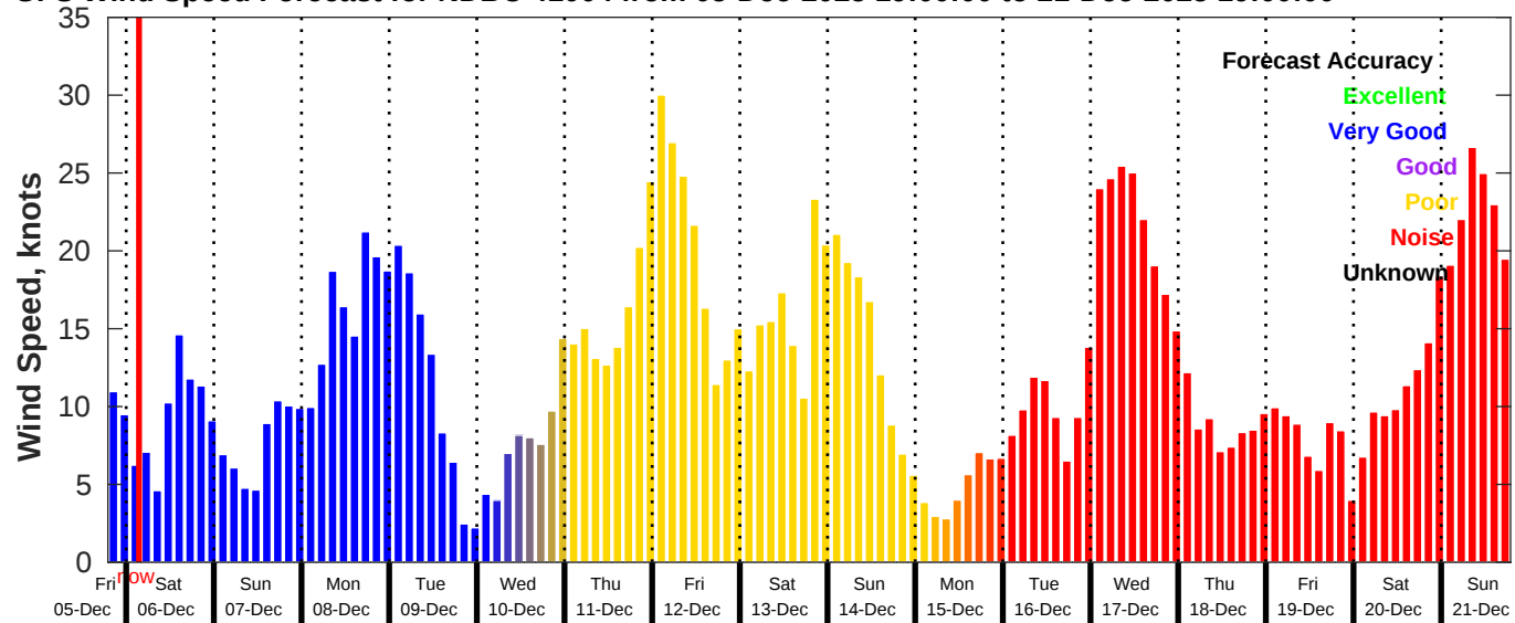
GFS Wind Speed Forecast for NDBC 41004 from 05-Dec-2025 19:00:00 to 21-Dec-2025 19:00:00
