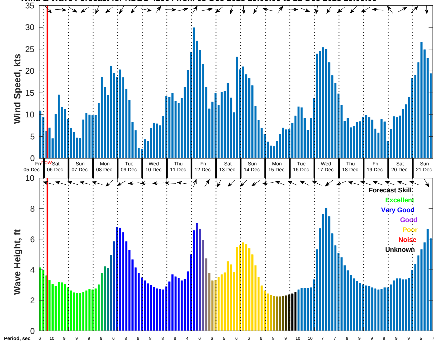
Wind & Wave Forecast for NDBC 41004 from 05-Dec-2025 19:00:00 to 21-Dec-2025 19:00:00
