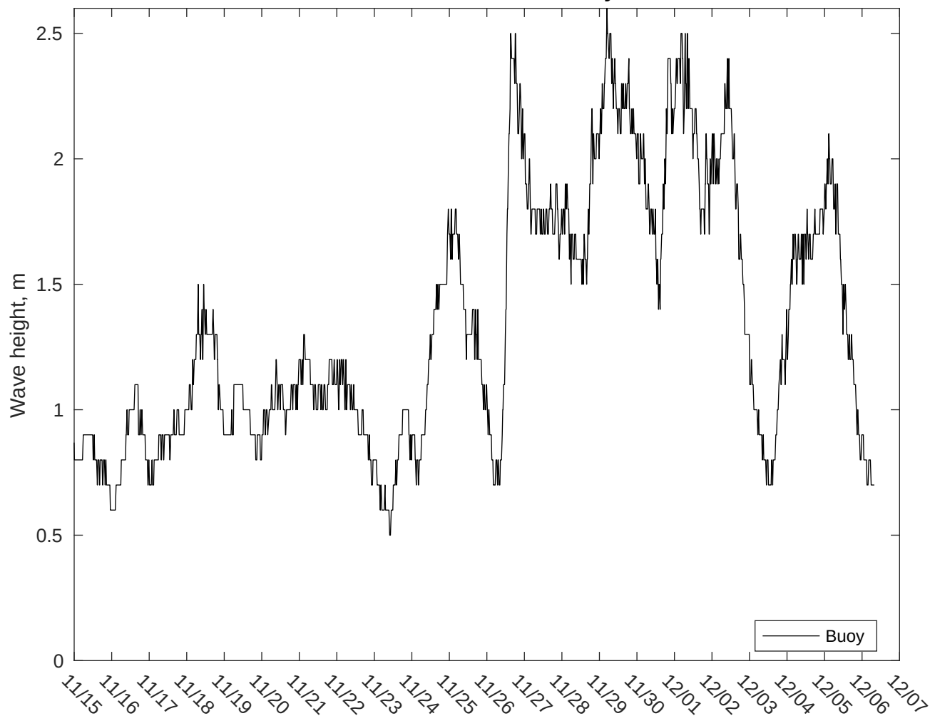
NDBC 42019 vs CMEMS Waves: 10 to 16 day forecast
